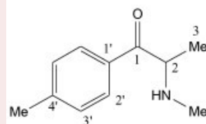
4-Methylmethcathinone (1)
